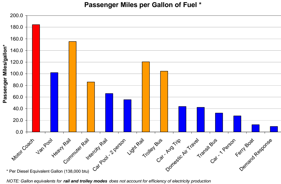
Figure 1.1 Passenger-Miles per Gallon of Fuel, by Mode
