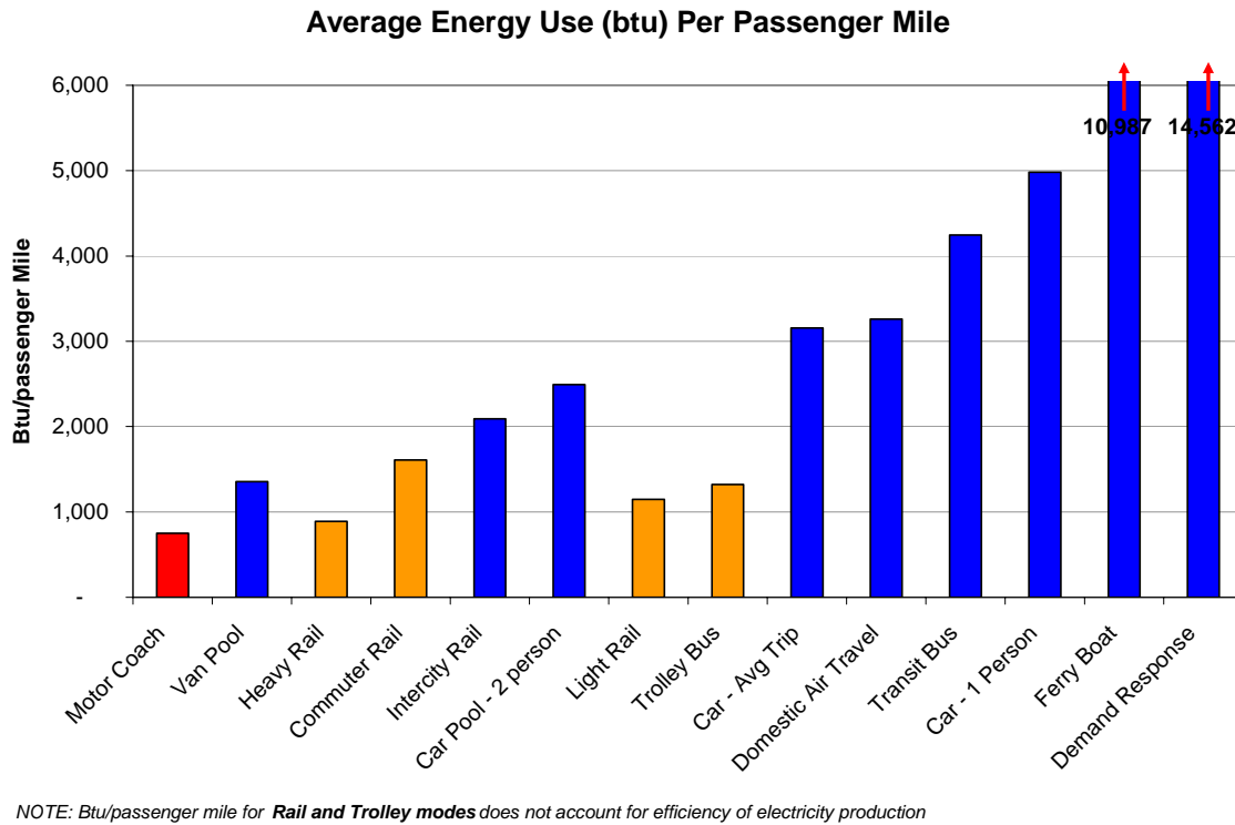
Figure 1.2 Energy Use (btu) per Passenger-Mile, by Mode
